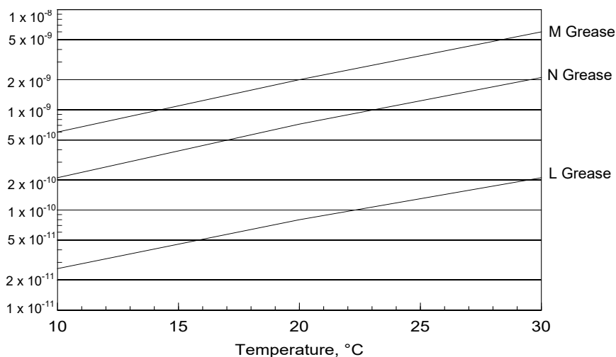
Vapour pressure over working temperature range
